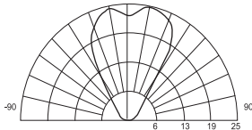
CANDLE POWER DISTRIBUTION FOR LEDEQMRM
